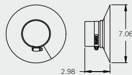
2SVSLSF03 Top Support/Storm Collar 3"
