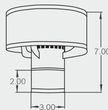
2SVSHRC03 3" Vertical Termination
