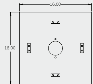
2SVSFSSF03 3" Firestop Support
