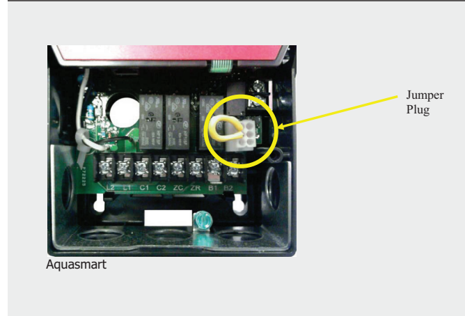
Fig. 2 Jumper plug location inside Aquasmart control
