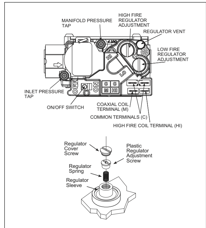
Figure 3 Gas Valve
