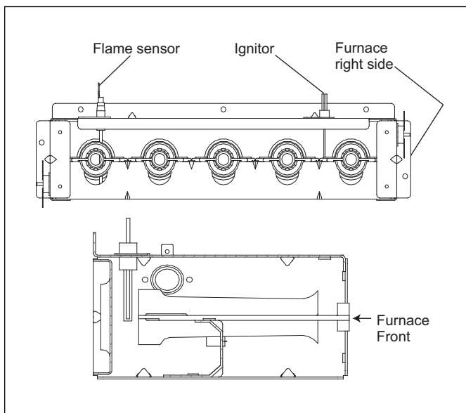
Figure 2 Ignitor Position
