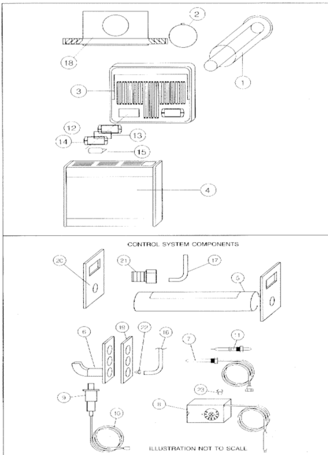
Fig. 14 - Required replacement parts for the EcoTherm
